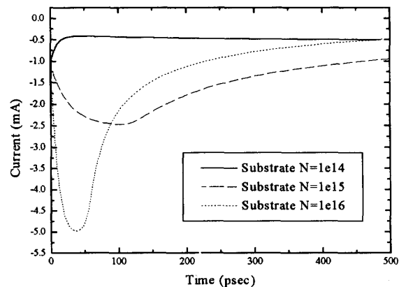
Figure 5. Responses to Changing Substrate Doping
