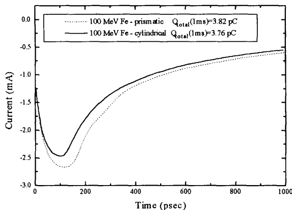
Figure 1. Prismatic and Cylindrical Mesh Simulations
