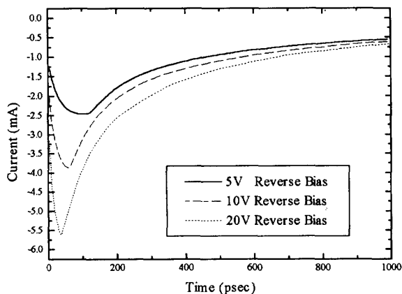
Figure 4. Responses to Changing Substrate Bias
