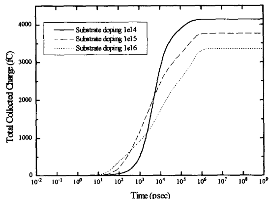
Figure 6. Charge as a Function of Substrate Doping
