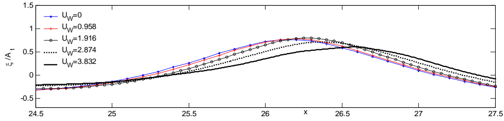
Fig. 15 Free surface profile near the crest at \tau \approx 61.85 in the cases with different wind speeds ( \omega_{min}=0.5 , \omega_{max}=1.4 , x_f=10 , \tau_f=31.32 , N=32 , a_n=0.008 )
