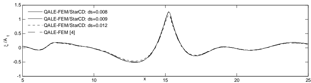
Fig.8 Free surface profiles recorded at at \tau \approx 41.49 in the case with different mesh sizes ( U_w=0 , \omega_{min}=0.5 , \omega_{max}=1.4 , x_f=10 , \tau_f=31.32 , N=32 , a_n=0.008 )
