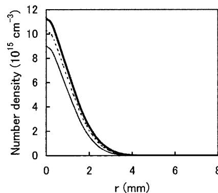
FIG. 7. Number density of mercury ions at three axial positions as a function of radial distance at the maximum current.
