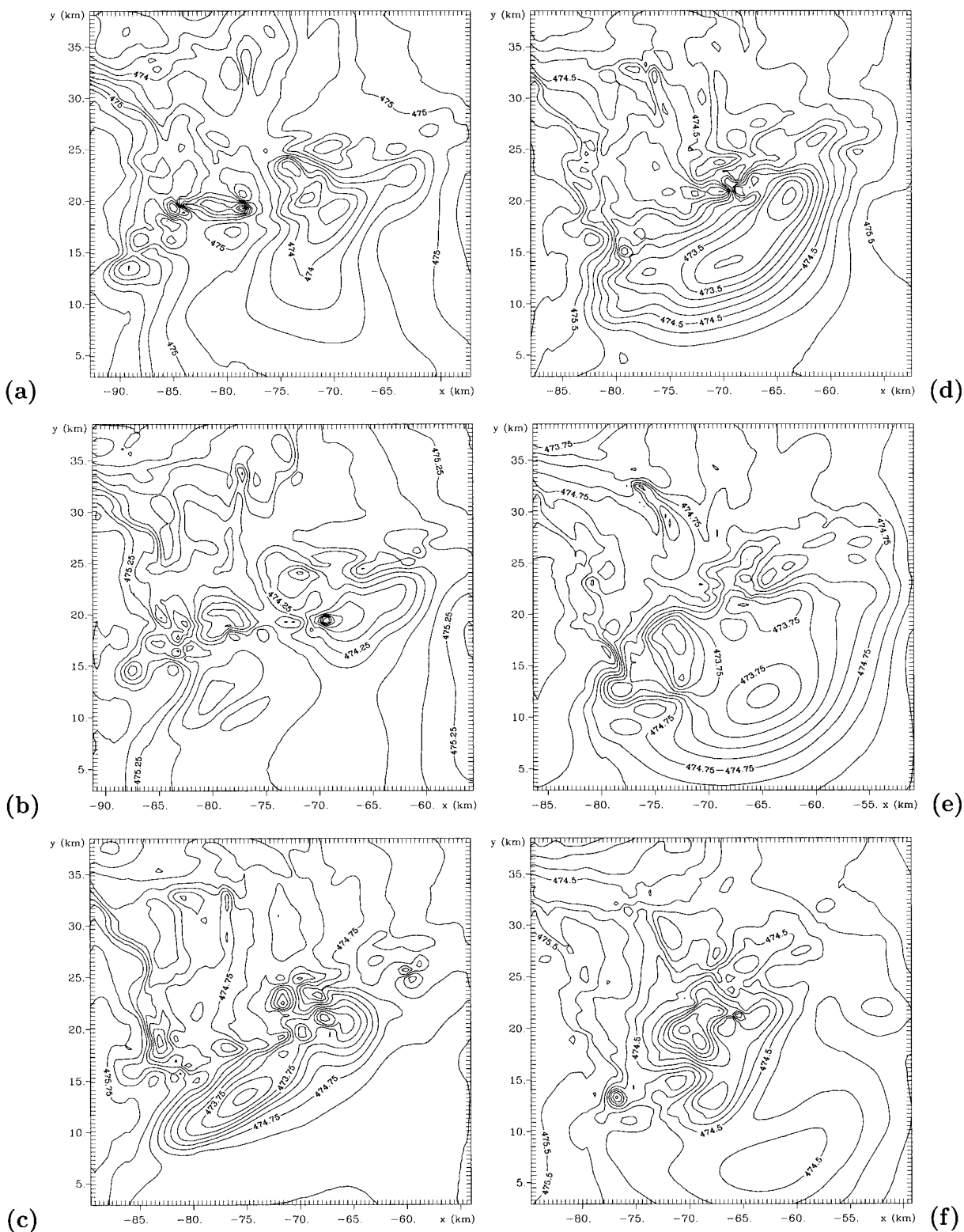
FIG. 13. Evolution of the pressure field (contour interval 0.25 mb) on grid 4 6.1 km above the surface at (a) 0013:30 UTC, (b) 0016:30 UTC, (c) 0019:30 UTC, (d) 0022:30 UTC, (e) 0025:30 UTC, and (f) 0028:30 UTC. Note the large gravity wave that propagates away from the storm between 0020 and 0030 UTC.
