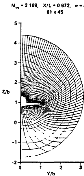
Fig 2 Elliptic grid at X/L = 0.672 and \alpha = 4^\circ
