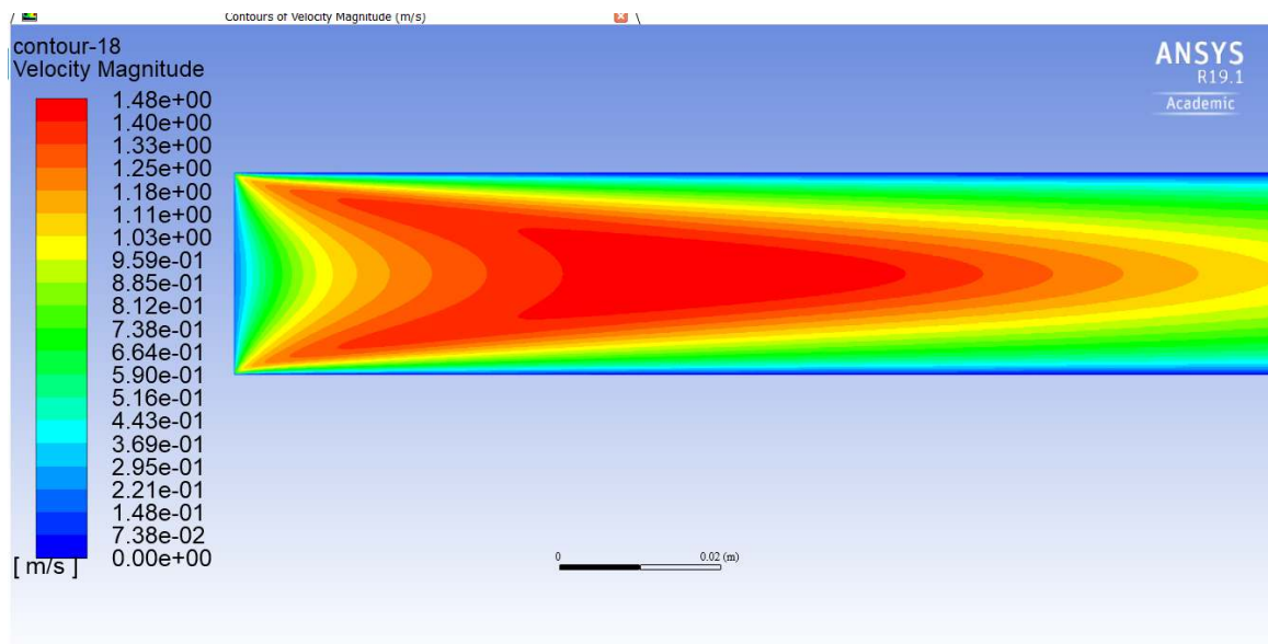
Figure 4-10 Velocity magnitude of the flow during the combustion
