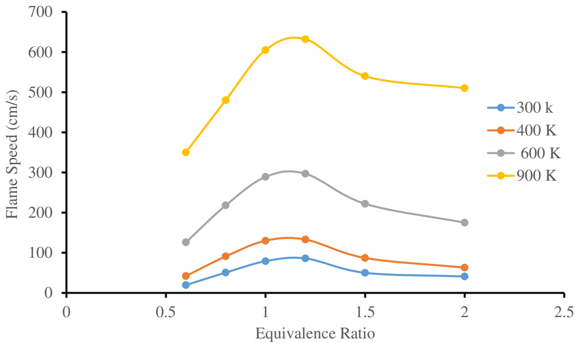
Figure 4-56 COG flame speed at different preheat temperature and \phi .
