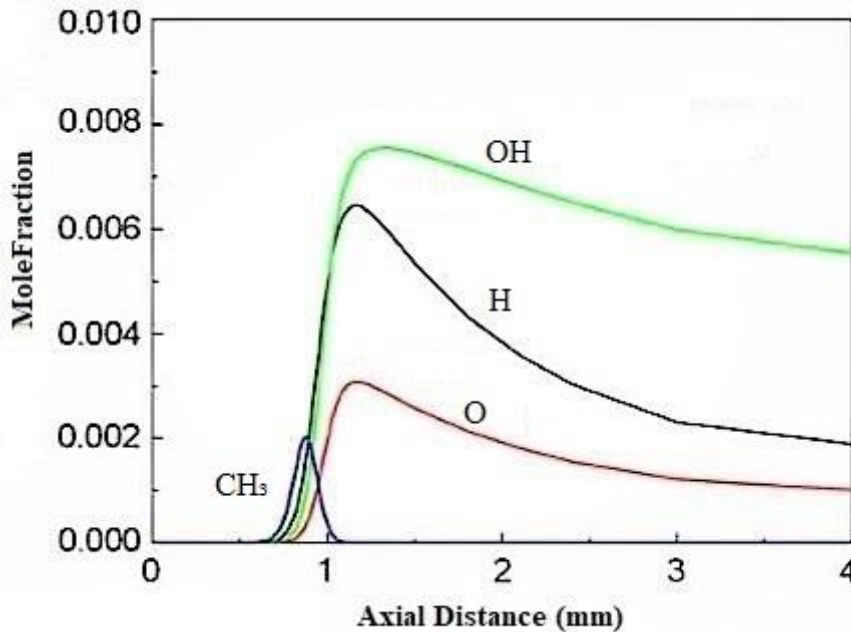
Figure 4-18 Methane air flame structure showing minor species.
