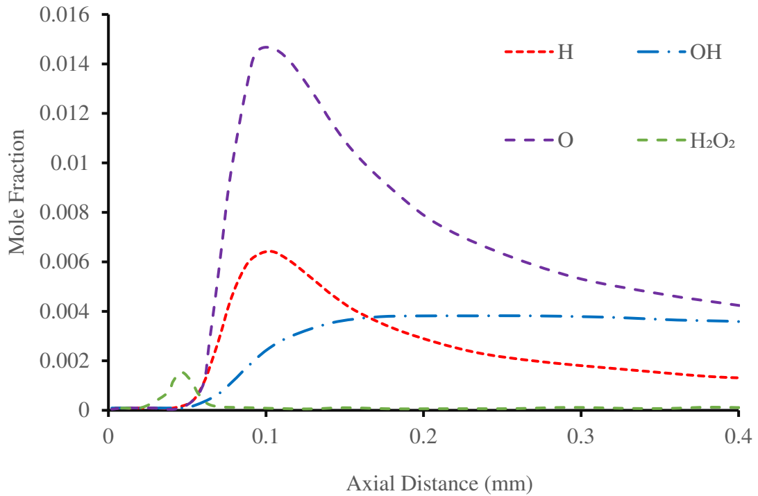
Figure 4-49 The radical formation in the case of 5/95 syngas at stoichiometry.
