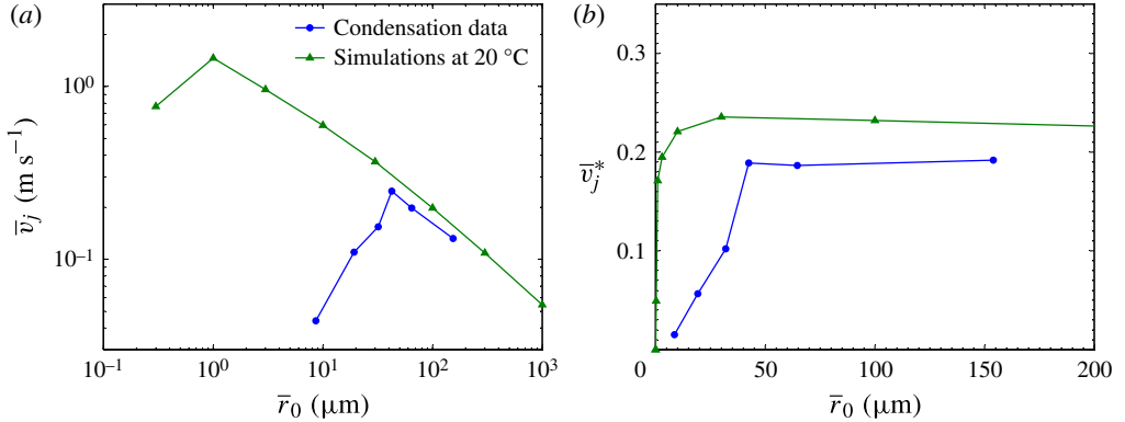
FIGURE 12. (Colour online) Comparison of numerical simulations at 20 °C with superhydrophobic jumping experiments. The experimental data are taken from Boreyko & Chen (2009), excluding asymmetric coalescence cases with larger than 33% disparity in the radii of coalescing drops. (a) The \bar{v}_j \sim \bar{r}_0^{-1/2} power law is parallel to the diagonal line of the logarithmic graph. The viscous cutoff radius is numerically predicted to be around 0.3 \mu\text{m} . (b) The same data are replotted on a linear graph emphasizing the region around 30 \mu\text{m} , the experimentally identified cutoff radius on textured superhydrophobic surfaces.
