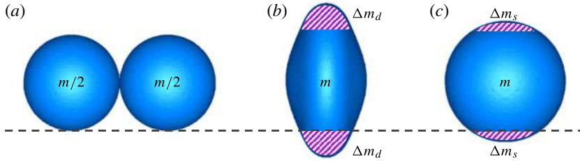
FIGURE 14. (Colour online) The symmetry-breaking action of the substrate can be estimated by the drop coalescence cases in the air. (a) Coalescence of two static drops of initial radius r_0 , each with a mass of m/2 . (b) For the maximum capillary–inertial deformation of the merged drop ( t^* = 2.36 in figure 3b), the dynamic crossing mass that passes below the imaginary substrate is \Delta m_d = 9.4\% m . (c) For an equilibrium drop, the static crossing mass is \Delta m_s = 3.0\% m . Note that the unbalanced counter-mass associated with the broken symmetry is also labelled.
