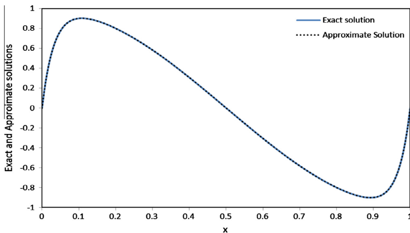
Figure 2 Exact and Approximate solutions for example1 at \epsilon_d = 10^{-3} and \epsilon_c = 10^{-6} .
