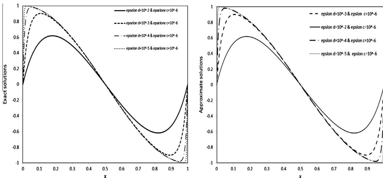
Figure 1 Exact and approximate solutions for example1 at different values of \epsilon_d = 10^{-2}, 10^{-4}, 10^{-3}, 10^{-5} and for fix \epsilon_c = 10^{-6} .
