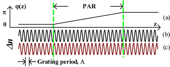
Fig. 1. (a) Phase distribution of a grating in a CPM DFB laser. The \pi -phase shift is distributed linearly in the PAR. (b) Index modulation of a grating with a uniform period of \Lambda . (c) Grating in the CPM DFB laser. It can be seen that the grating has a \pi -phase difference at the right side compared with the uniform grating.
