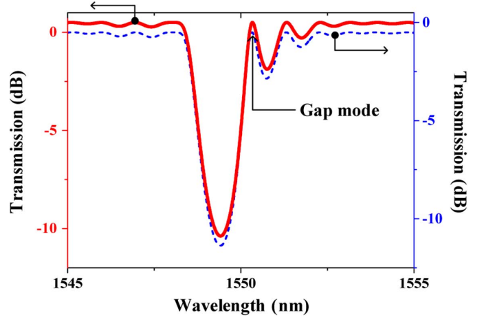
Fig. 3. Transmission spectra of the regular chirp grating (dotted line) and the SBG with an equivalent chirp at the -1 st channel (solid line) around 1550 nm. Identical spectral characteristics are observed.
