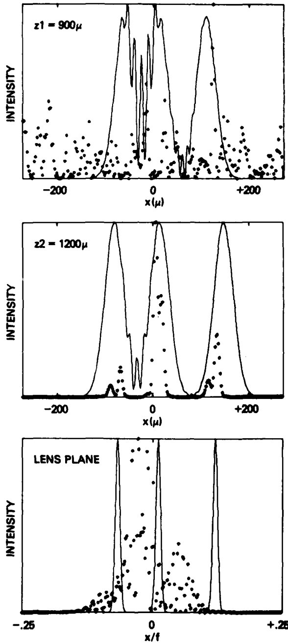
Fig. 12 - Transverse profiles for a 300\mu plasma of density .2 n_c \exp \{-(z - 900)/100\} , illustrating that small scale retrace disappears when the pump beams do not overlap.
