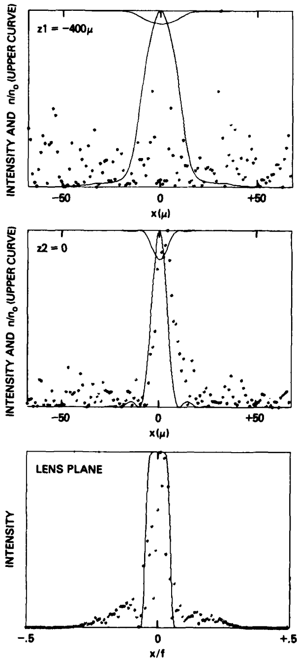
Fig. 7a - Transverse profiles for a uniform 400 plasma located just beyond the focal plane z_2 = 0 . [Below threshold for retrace ( B = 1.2 , \Delta n G = 1.3 ) with n_0 = .01 n_c ]
