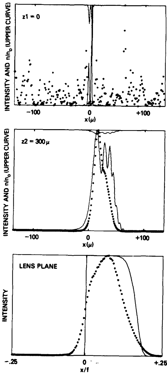
Fig. 6b - Transverse profiles of the pump radiation and backscatter from a 300\mu plasma of density .2 n_c \exp(-z/100) , showing partial retracing of a half blocked pump beam at the lens. The stochastic noise appears as random dots at the focal plane z_1 = 0 . [Strong self focusing ( B = 7.6 ) with comparable gain \ln G = 8.9 ] The density variations n/n_0 are given by Eq. (15).
