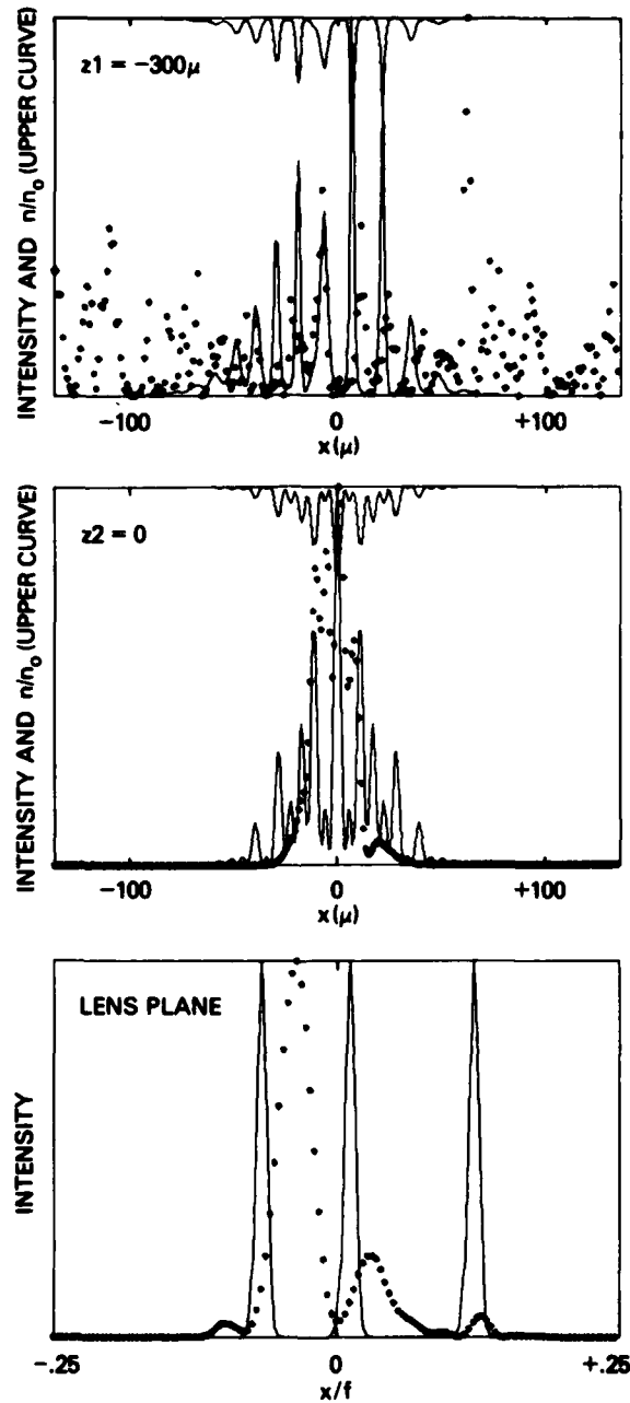
Fig. 11b - Transverse profiles for a 300\mu plasma of density .2 n_c \exp \{-(z + 300)/100\} , showing the degradation of small scale retrace by whole beam self focusing. ( B = 5.17 with \ln G = 9.4 )
