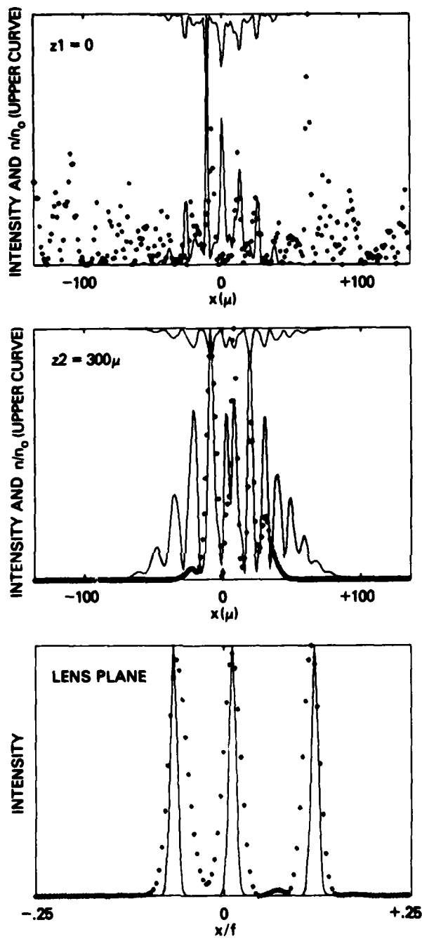
Fig. 10b - Transverse profiles for a 300\mu plasma of density .2 n_c exp (-z/100) , showing nearly complete retrace of the three pump beams at the lens. [Strong self focusing ( B = 5.6 ) with \ln G = 10 ]
