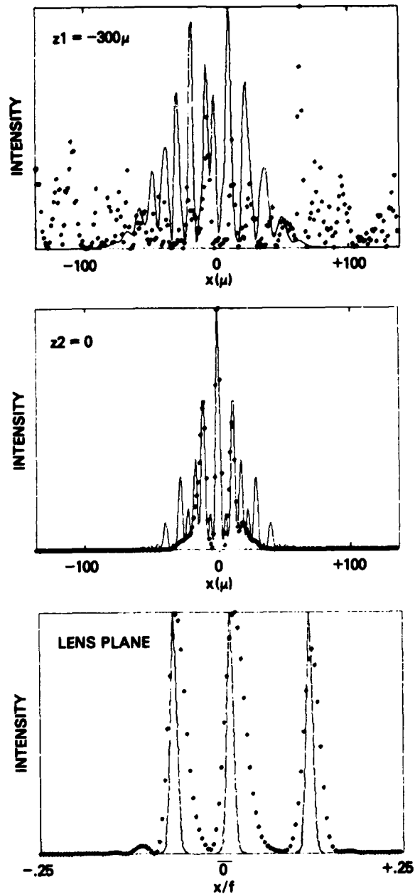
Fig. 11a - Transverse profiles for a 300\mu plasma of density .2 n_c \exp \{-(z + 300)/100\} . [Negligible self focusing ( B = 0 ) with \ln G = 12 ]
