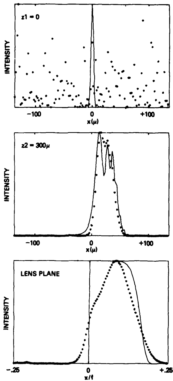
Fig. 6a- Transverse profiles of the pump radiation and backscatter from a 300\mu plasma of density .2 n_c \exp(-z/100) , showing partial retracing of a half blocked pump beam at the lens. The stochastic noise appears as random dots at the focal plane z_1 = 0 . [Negligible self focusing ( B = 0 ), with l_n G = 11 ]
