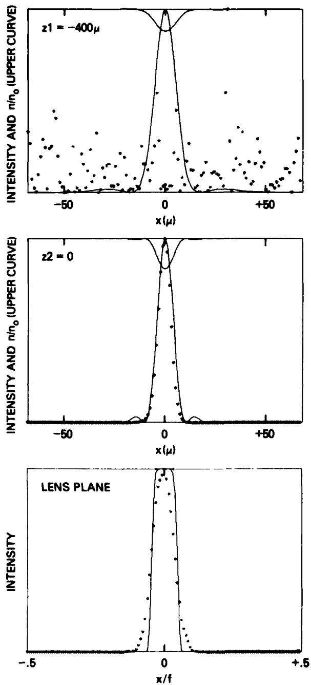
Fig. 7b - Transverse profiles for a uniform 400 plasma located just beyond the focal plane z_2 = 0 . [Above threshold ( B = 2.9 , \ln G = 7.3 ) with the same incident pump intensity, but n_0 = .02 n_c ]
