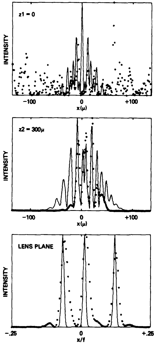
Fig. 10a - Transverse profiles for a 300\mu plasma of density .2 n_c \exp(-z/100) , showing nearly complete retrace of the three pump beams at the lens. [Negligible self focusing ( B = 0 ) with \ln G = 9.2 ]
