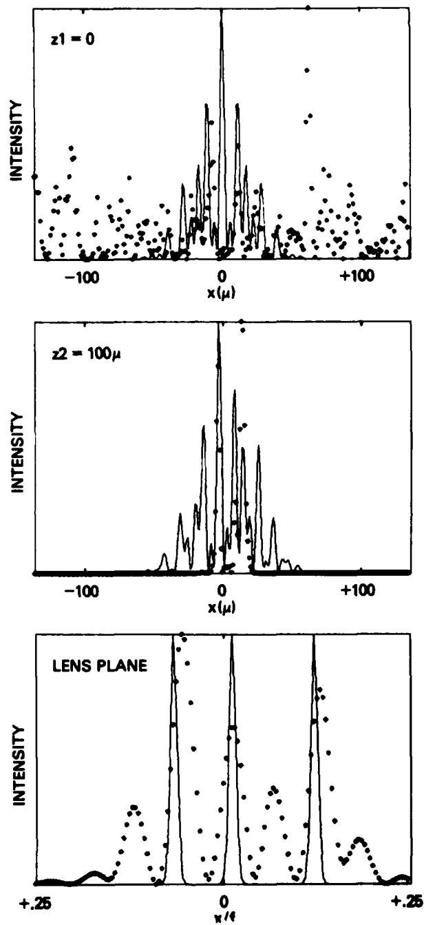
Fig. 9 - Transverse profiles for a uniform 100\mu plasma at the focal plane z_1 = 0 , showing partial retracing of the three pump beams at the lens. ( B = 0 , \ln G = 12.5 )
