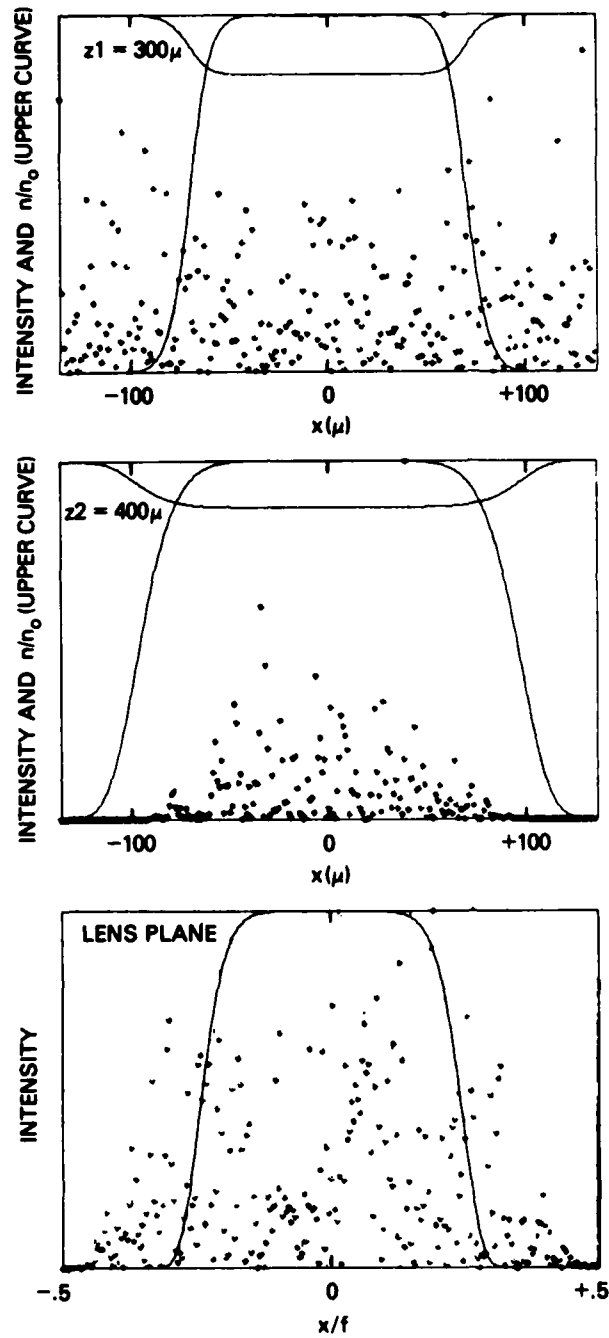
Fig. 8 - Transverse profiles for a uniform 100\mu plasma in the quasi near field of the lens. The whole beam ray retracing is ineffective when the width of the gain region becomes comparable to its length.
