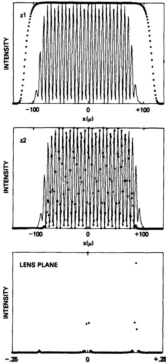
Fig. 4 - Transverse intensity profiles for two plane hyper-Gaussian pump waves ( \theta = 0 , \theta' = \theta_D = 0.16 radian) and a backscatter "noise" wave ( \theta_1 = 0 ) o interacting within a uniform 100 \mu plasma slab centered at z' = 0 . In this and all subsequent profiles, the solid and dotted lines are the normalized pump and backscatter intensities respectively.
