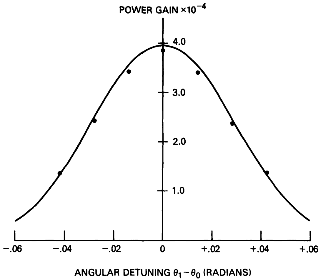
Fig. 5 - Tuning curve for the 100 \mu slab, showing Brillouin gain G vs. angular detuning \theta_1 - \theta_0 . The solid line is the analytic result from Refs. 11 or 24 0 (exact for infinite plane waves), and the dots are the numerical results from BOUNCE.
