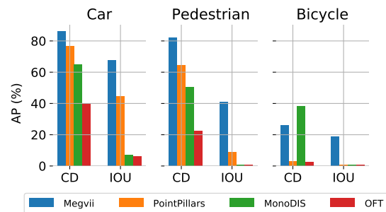
Figure 7. Average precision vs. matching function. CD: Center distance. IOU: Intersection over union. We use IOU = 0.7 for car and IOU = 0.5 for pedestrian and bicycle following KITTI [32]. We use CD = 2m for the TP metrics in Section 3.1.
