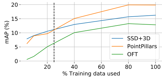
Figure 6. Amount of training data vs. mean Average Precision (mAP) on the val set of nuScenes. The dashed black line corresponds to the amount of training data in KITTI [32].
