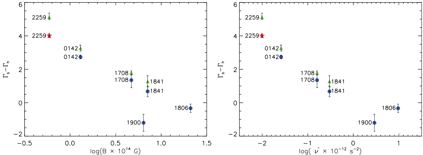
Figure 9. Spectral turnover ( \Gamma_s - \Gamma_h ) vs. magnetic field B (left) and spin-down \dot{\nu} (right) from Kaspi & Boydstun (2010) for all magnetars presented there as well as our new result. Blue circles represent total flux, and green triangles represent pulsed flux. Our total flux result is indicated by the red star. 1\sigma uncertainties are shown. For details on the full list of magnetar names, included data, and references, see Kaspi & Boydstun (2010).
