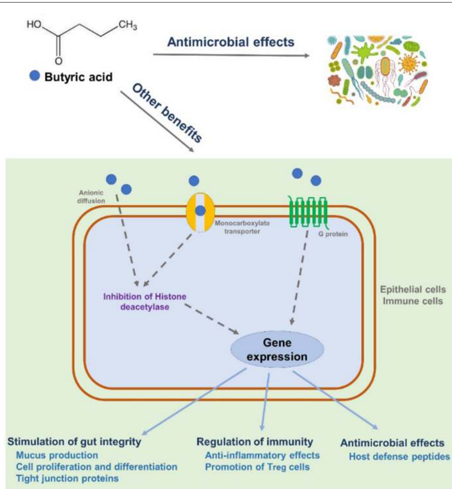
FIGURE 2 | Proposed mechanisms of action on the beneficial effects of butyric acid.
