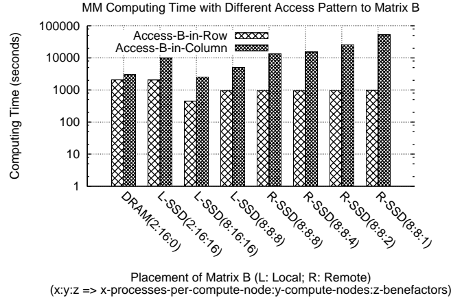
Figure 5. MM: Row-major versus Column-major for 2GB/matrix.
