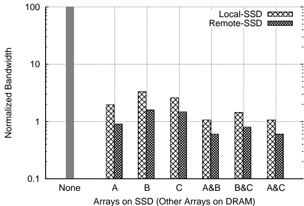
Figure 2. Bandwidth of STREAM TRIAD. Y-axis is normalized to show DRAM bandwidth as 100. Note that a logarithmic scale is used for the Y-axis. X-axis shows which arrays are on the NVM. “None” indicates all arrays are on DRAM.
