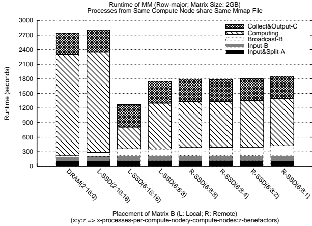
Figure 3. MM Runtime with Shared Mmap File for matrix B for a problem size of 2GB/matrix.
