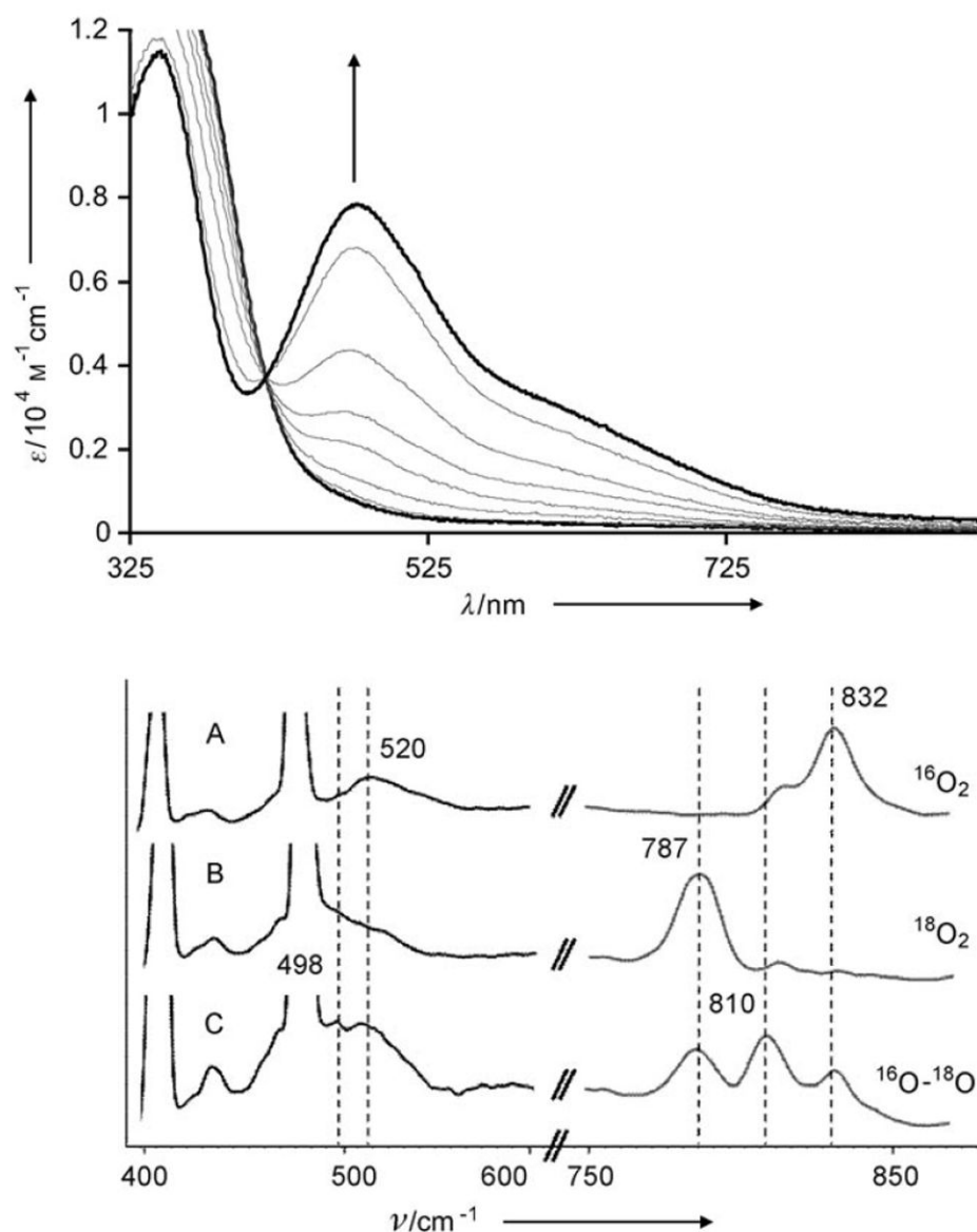
Figure 3. Top: UV/Vis spectra for the reaction of 1 -CF 3 SO 3 with O 2 in acetone at -90°C to form 1 -O 2 . Bottom: Resonance Raman spectra ( \lambda_{\text{ex}} = 488 \text{ nm} ) of frozen acetone solutions of 1 -O 2 from 16 O 2 (A), 18 O 2 (B), and 18 O 16 O (C).
