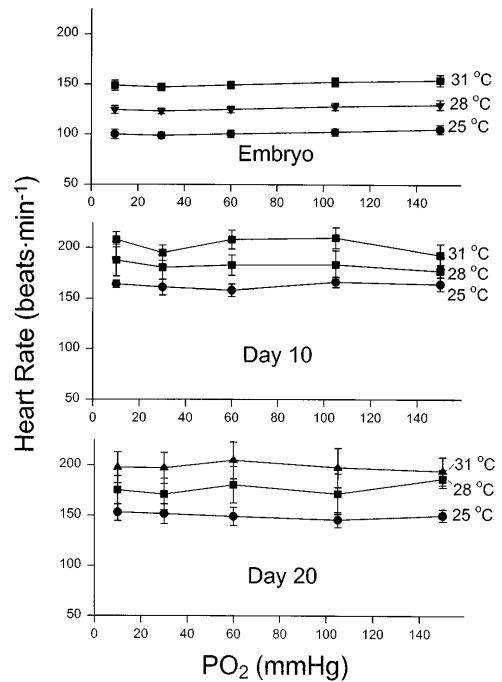
Fig. 6. Influence of acute hypoxic exposure on heart rate as a function of temperature in embryos and larvae (days 10, 20) of the zebrafish D. rerio . Mean values \pm SE are plotted; n = 10 for each plotted developmental stage at all 3 temperatures. See RESULTS for statistical assessment.
