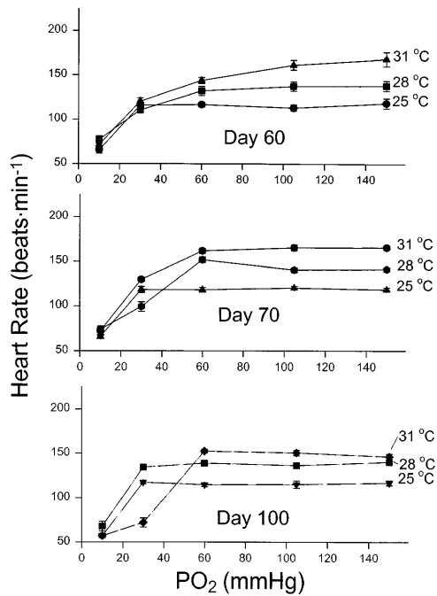
Fig. 8. Influence of acute hypoxic exposure on heart rate as a function of temperature in juveniles ( days 60, 70 ) and adults ( day 100 ) of the zebrafish D. rerio . Mean values \pm SE are plotted; n = 10 for each plotted developmental stage at all 3 temperatures. See RESULTS for statistical assessment.
