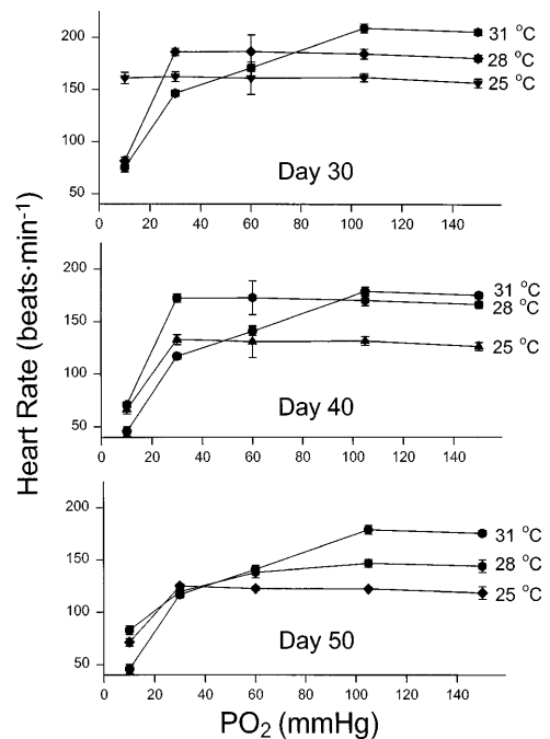
Fig. 7. Influence of acute hypoxic exposure on heart rate as a function of temperature in juveniles (days 30, 40, and 50) of the zebrafish D. rerio . Mean values \pm SE are plotted; n = 10 for each plotted developmental stage at all 3 temperatures. See RESULTS for statistical assessment.
