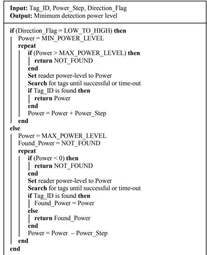
Figure 2. Algorithm I: Linear search for the minimum power-level
