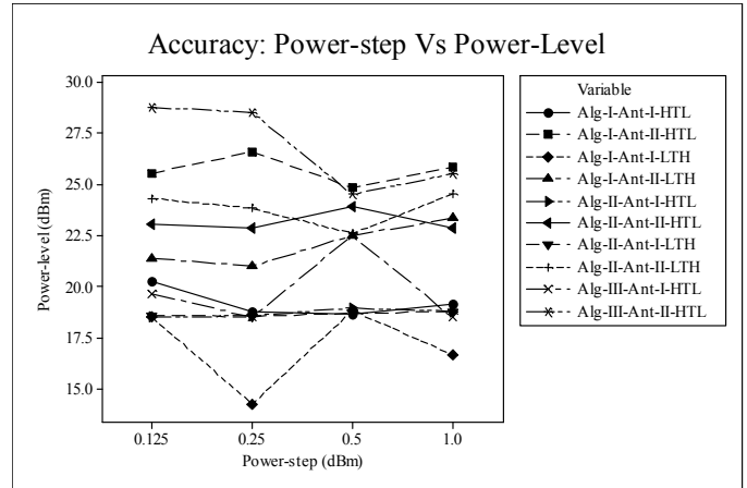
Figure 6. Power level comparison for algorithms I, II, and III
