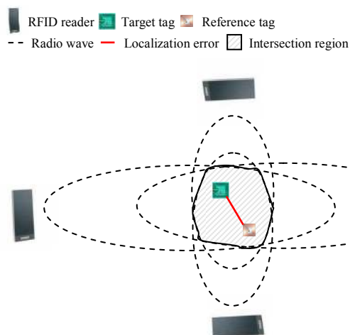
Figure 1. Working principle of the proposed localization method
