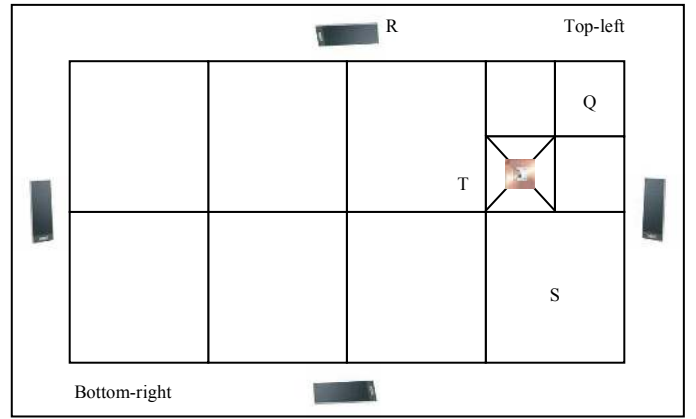
Figure 3. The experimental region with sectors (S), quadrants (Q), reference tags (T), and reader antennas (R)
