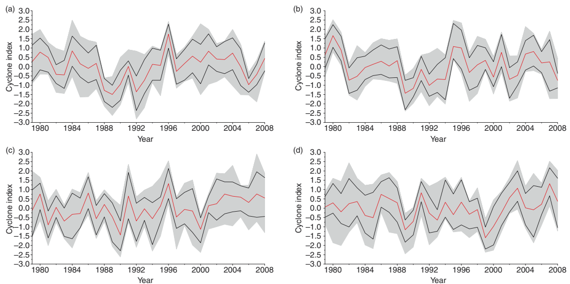
Fig. 10. Time series of cyclone number index for the four sectors of the Mediterranean region. (a) NW, (b) NE, (c) SW and (d) SE. The central red line shows the MTCMmean, the lower and upper black lines show the 10th and 90th percentiles of the CDTM results, and the whole grey area corresponds to the spread of the data.
