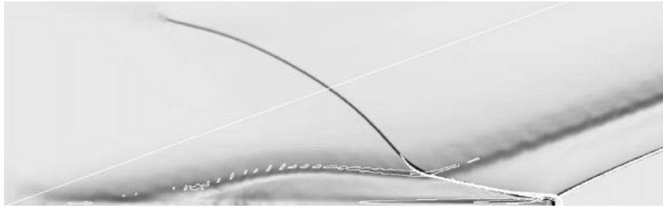
t = 5.35 and 10.84 , \alpha = 20^\circ
