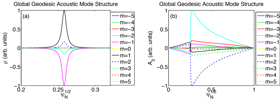
Figure 2: Eigenmode structure of the global geodesic acoustic mode found slightly above the peak in the geodesic acoustic wave continuum, located at \sqrt{\psi_N} = 0.26 , for a reversed shear, circular JET-like equilibrium. (a) The perturbed mass density and (b) the perturbed parallel vector potential.
