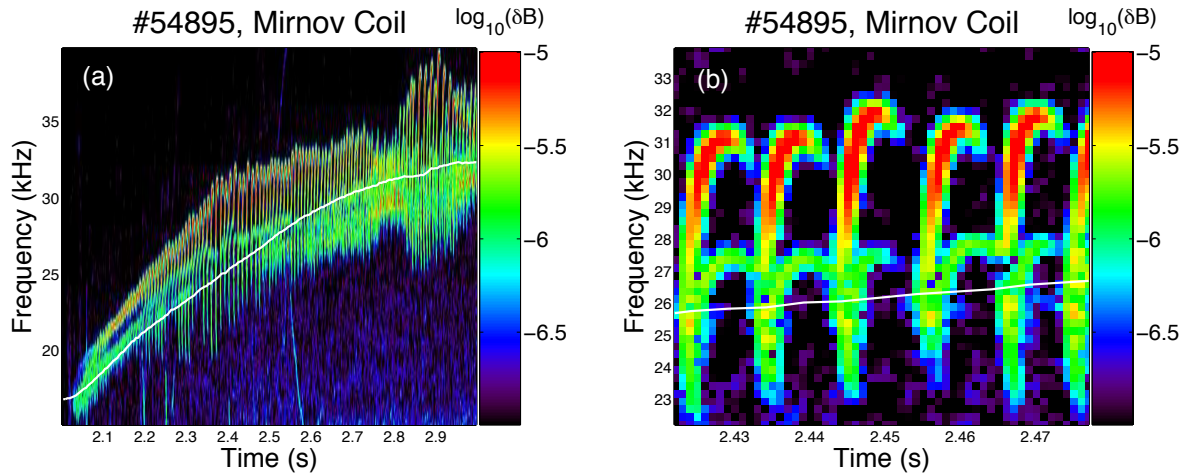
Figure 1: Spectrograms of the signal from a Mirnov coil on JET. (a) The rapidly chirping n=0 mode. (b) A zoom of (a) showing the frequency chirping in more detail. In both plots the white line is proportional to \sqrt{T_e(r/a = 0.15)} .
