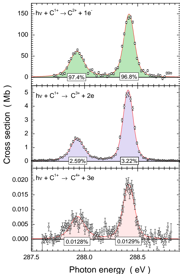
FIG. 4. (color online) Cross section for single, double and triple ionization of ground-state C^{1+} ions by single photons with 92 meV bandwidth. The resonances seen in all the observed channels are associated with K -shell-excited C^{1+}(1s2s^22p^2D,^2P) terms. The percentages given for the areas of the peaks indicate the branching factors for single-, double-, and triple-Auger decay.
