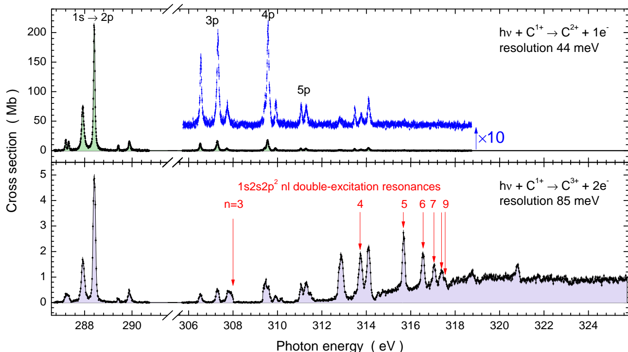
FIG. 2. (color online) Absolute cross sections for single and double ionization of C^{1+} ions by single photons. The photon energy axis has a break in the range where no resonances are expected. The experimental data are shown as small dots with statistical error bars. They are connected by a solid line with shading. The cross section data for single ionization in the high-energy region were multiplied by a factor of 10 and displayed again with a vertical offset. Important resonance groups are identified by their configurations.
