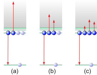
FIG. 1. (color online) Single- (a), double- (b) and triple-Auger (c) decay of a K -shell excited B-like atom.
