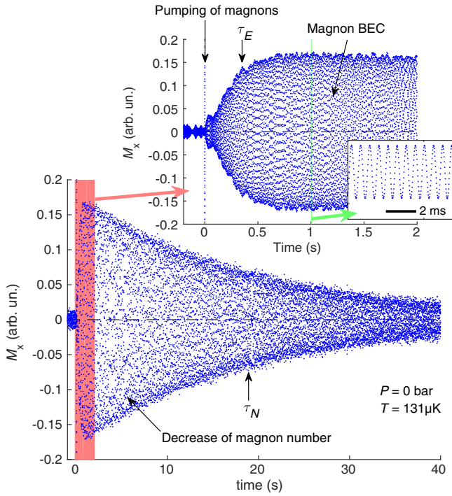
FIG. 1. Time supercrystal in superfluid {}^3\text{He-B} emerging from spontaneous coherence in freely precessing magnetization. (Top) The coherent precession of magnetization, M_x + iM_y = \gamma S_\perp e^{i\omega t} , is established with time constant \tau_E after the excitation pulse at t = 0 . The signal is picked up by the NMR coils (Fig. 2) and down-converted to lower frequency (with reference at 834 kHz). (Bottom) Since the magnetic relaxation in superfluid {}^3\text{He} is small, the number of magnons N slowly decreases with timescale \tau_N \gg \tau_E . During relaxation the precession remains coherent, and the state represents Bose-Einstein condensate of magnons until the number of magnons drops below the critical value (which in these experiments corresponds to a signal below the noise level).
