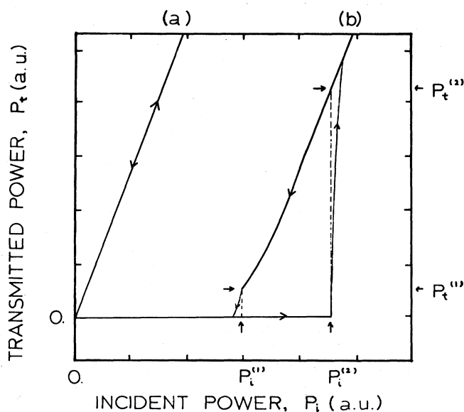
FIG. 2. x - y oscilloscope traces of transmitted laser power P_t vs incident laser power P_i for zero atomic and cavity detunings. (a) No intracavity atomic beams. (b) Intracavity beams with resonant absorption \alpha_m l = 1.13 and with P_i^{(1)} = 70 \mu\text{W} , P_i^{(2)} = 104 \mu\text{W} .
