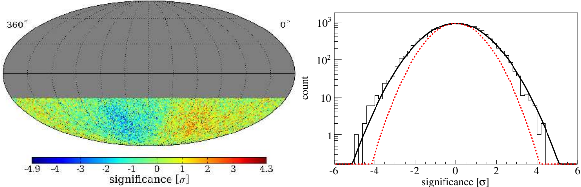
Fig. 3.— Left : Significance sky map of the IC59 data in equatorial coordinates, produced using a time window of 24 hours. Right : 1d-distribution of the significance values together with the best-fit (black solid line) performed with a Gaussian function. For comparison, a Gaussian function of mean zero and unit variance (red dashed line), expected from an isotropic sky, has been superimposed.
