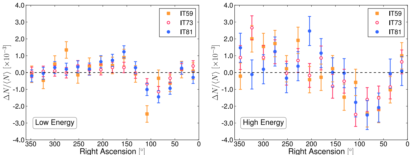
Figure 9. Relative intensity as a function of right ascension for the low-energy (left) and high-energy (right) data samples in the declination band -75^\circ < \delta < -35^\circ for the three detector configurations of IceTop considered in this work (IT59, IT73, and IT81). For clarity, only statistical error bars are shown.
