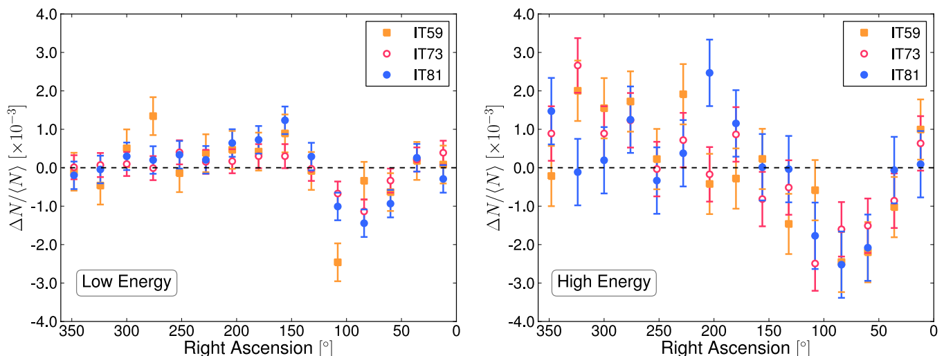
Figure 9. Relative intensity as a function of right ascension for the low-energy (left) and high-energy (right) data samples in the declination band -75^\circ < \delta < -35^\circ for the three detector configurations of IceTop considered in this work (IT59, IT73, and IT81). For clarity, only statistical error bars are shown.
