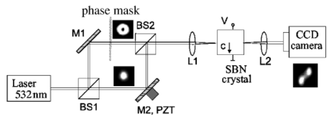
FIG. 2. Experimental setup.
