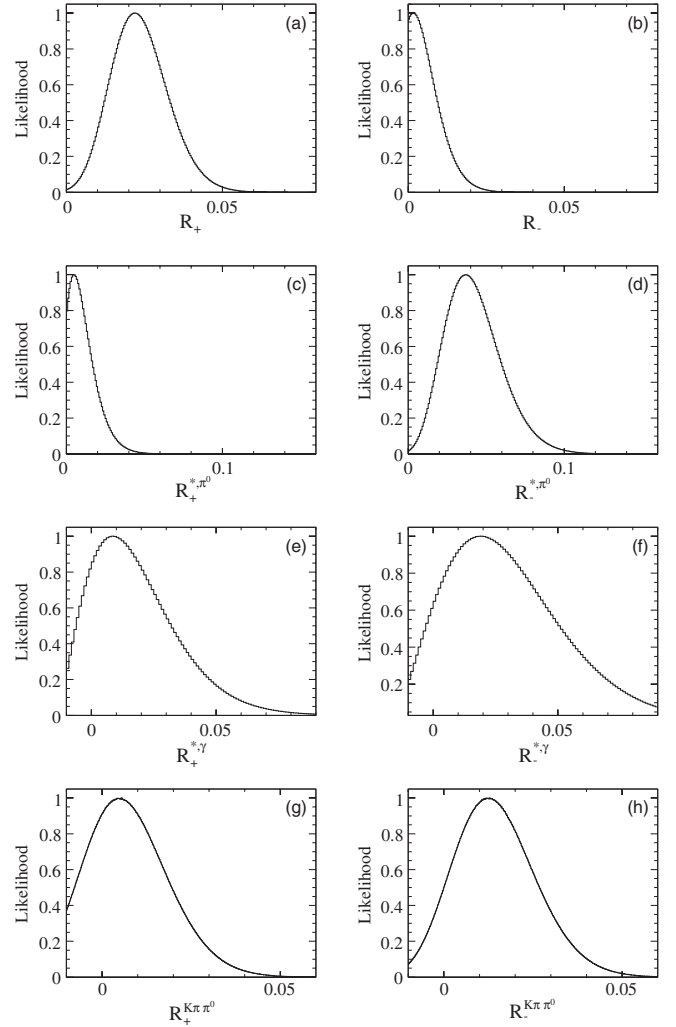
FIG. 2. Experimental likelihoods as functions of the ADS charge-specific ratios R_{\pm} (a,b), R_{\pm}^* [D\pi^0] (c,d), R_{\pm}^* [D\gamma] (e,f), and R_{\pm}^{K\pi\pi^0} (g,h), from Refs. [23,24], including systematic uncertainties. The P.D.F.s are normalized so that their maximum values are equal to 1. These distributions are well parametrized by sums of two asymmetric Gaussian functions with mean values as given in Table III.
