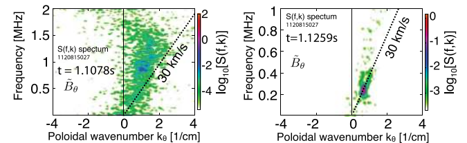
FIG. 5 (color online). Frequency vs wave number spectra of the magnetic fluctuations for two distinct time slices; [Left]: before the onset of instability and [right]: saturated regime. In both panels, an oblique lines is displayed to show the corresponding phase velocity of 30 km/s.
