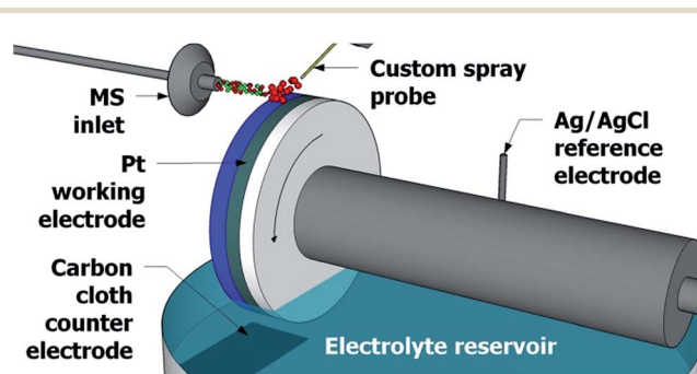
Fig. 1 The setup used for detection of electrochemical reaction intermediates, employing a rotating waterwheel electrode. Wheel rotation is indicated by the curved arrow.
