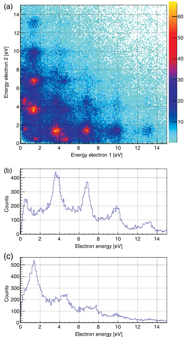
FIG. 3 (color online). Double ionization of Ar by 394 nm, 45 fsec pulses. Same laser conditions as in Fig. 2. (a) Energy of one electron versus the energy of the other electron. The electrons are integrated over all angles. (b) Energy of one of the electrons if the other electron has an energy between 1.0 and 1.6 eV, i.e., projection of (a) in the range 1.0–1.6 eV. (c) Same as (b) for the range 3.0–3.8 eV.
