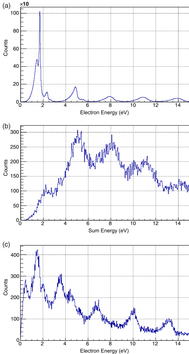
FIG. 2 (color online). (a) Electron energy distribution for single ionization of Ar at 394 nm, 1.3 \times 10^{14} \text{ W cm}^{-2} (marked with the red arrow in Fig. 1). (b) Sum of the energy of both electrons from double ionization of Ar at the same conditions as (a). (c) Energy of one of the two electrons from double ionization.
