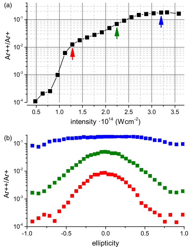
FIG. 1 (color online). Ratio of double to single ionization of Ar by 394 nm, 45 fsec laser pulses (a) as a function of laser intensity and (b) as function of polarization ellipticity at the intensity marked by colored arrows in (a). The intensity shown by the red arrow was used in the experiment ( 1.3 \times 10^{14} \text{ W cm}^{-2} ). Note the logarithmic scale.
