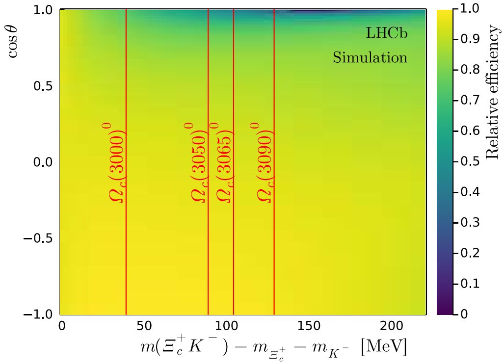
Figure 8: Efficiency map in the [\Delta M, \cos \theta] plane. Positions of the four narrow \Omega_c^{**0} states are shown by the red lines.
