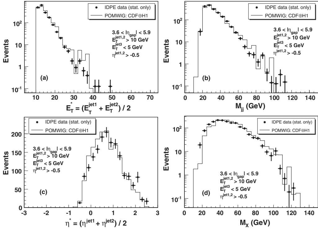
FIG. 12. Comparison of IDPE data distributions of (a) E_T^* , (b) M_{jj} , (c) \eta^* , and (d) M_X for the background-rich region B with corresponding POMWIG distributions obtained using the CDF \oplus H1 DSF; the events plotted are those used in plots (a) and (b) of Fig. 11.
