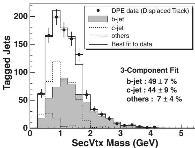
FIG. 21. Displaced secondary vertex mass distribution for jets tagged by the SECVTX algorithm in DPE data (points). The solid histogram shows the result of a three-component maximum likelihood fit to the data, using Monte Carlo templates of distribution shapes, consisting of b -jets (shaded histogram), c -jets (dashed histogram), and other jets (dotted histogram) obtained from PYTHIA dijet events.
