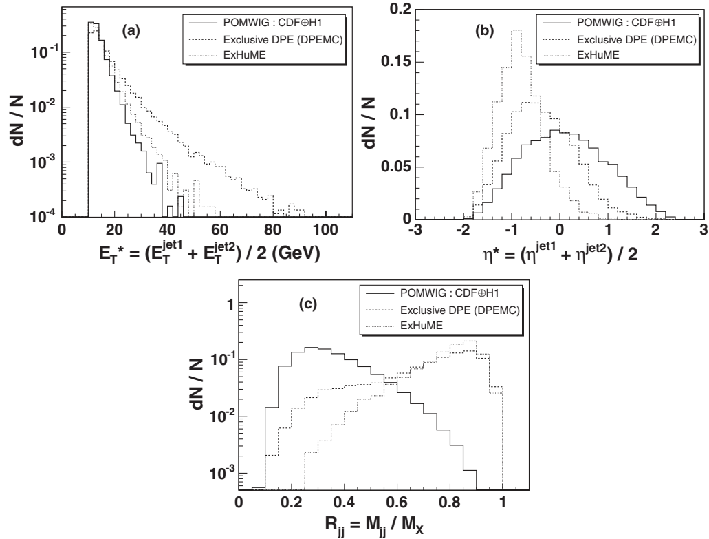
FIG. 13. (a) Mean E_T^{\text{jet}} of the two leading jets, E_T^* , (b) mean \eta^{\text{jet}} , \eta^* , and (c) dijet mass fraction, R_{jj} for POMWIG DPE dijet events generated using the CDF \oplus H1 DSF diffractive/Pomeron structure function (solid histograms), and for exclusive dijet events generated with the EXCLDPE (dashed histograms) and EXHUME MC simulations (dotted histograms). All distributions are normalized to unit area.
