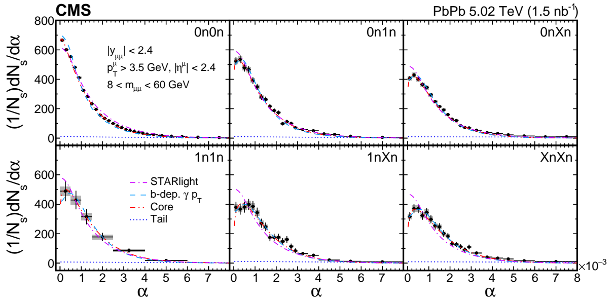
Figure 3: A direct comparison between data and model calculations for the \alpha distributions with \alpha < 0.008 . The dot-dashed line shows the STARLIGHT prediction and the dashed line corresponds to the leading-order QED calculation of Ref. [48]. The dot-dot-dashed and dotted lines indicate the core and tail contributions, respectively. The vertical lines and shaded areas represent the statistical and systematic uncertainties, respectively.
