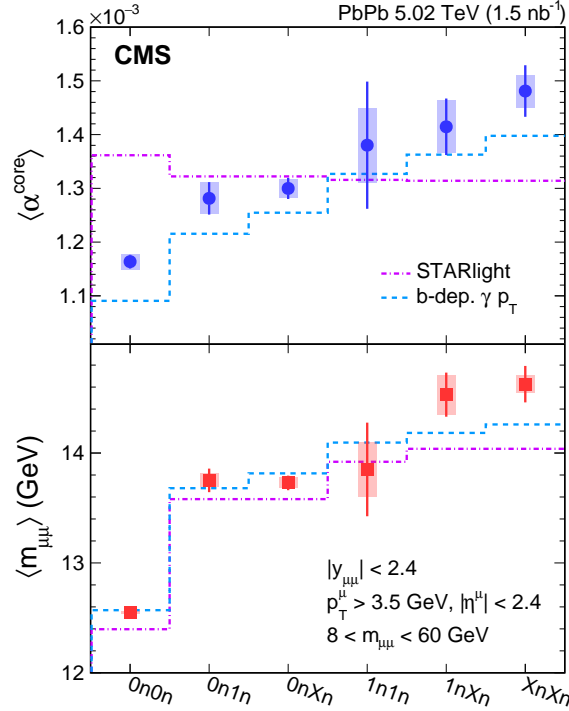
Figure 2: Neutron multiplicity dependence of (upper) \langle\alpha^{\text{core}}\rangle and (lower) \langle m_{\mu\mu}\rangle of \mu^+\mu^- pairs in ultraperipheral Pb-Pb collisions at \sqrt{s_{\text{NN}}} = 5.02 TeV. The vertical lines on data points depict the statistical uncertainties, while the systematic uncertainties of the data are shown as shaded areas. The dot-dashed line shows the STARLIGHT prediction, and the dashed line corresponds to the leading-order QED calculation of Ref. [48].
