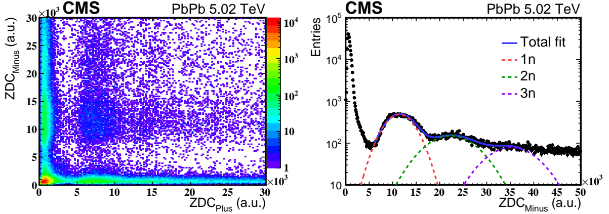
Figure A.1: The left panel shows the correlation between energy distributions of the Minus and Plus ZDC detectors (one entry per event), while the right panel shows a multi-Gaussian function fit to the Minus ZDC energy distribution.
