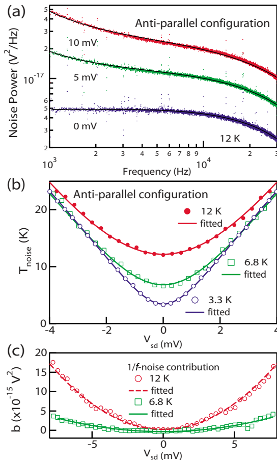
FIG. 3. (Color online) (a) Noise spectral density S_V(f) for the AP magnetization configuration at V_{sd}=0, 5, and 10 mV. (b) Noise power as a function of bias voltage expressed in terms of the noise temperature T_{noise} . (c) 1/f contribution as a function of V_{sd} .
