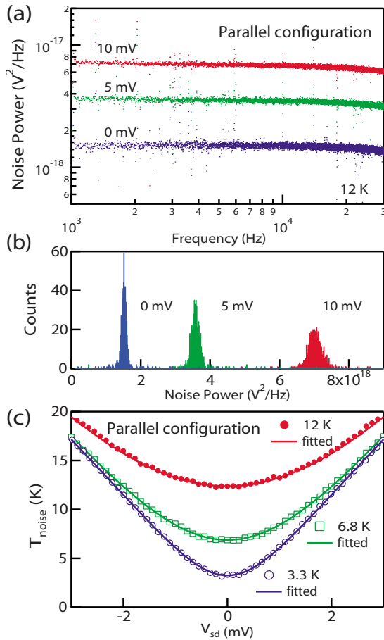
FIG. 2. (Color online) (a) Noise spectral density S_V(f) for the P magnetization configuration at V_{sd}=0, 5, and 10 mV. (b) Histograms of the noise power spectral density between 1 and 5 kHz. (c) Noise power as a function of bias voltage expressed in terms of the noise temperature T_{\text{noise}} .
