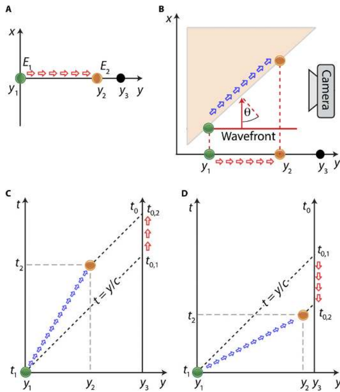
Fig. 1. (A) An illustration of the (1 + 1)D example described in the text. (B) The extension of (A) to a (2 + 1)D case that exemplifies the experimental layout. The motion of the scattering source toward the observer (red arrows) can be either superluminal or subluminal. (C) Minkowski diagram for two sequential events. Because this case has v < c , time ordering is preserved. (D) Minkowski diagram for two (causally disconnected) events where v > c : time ordering is inverted.
