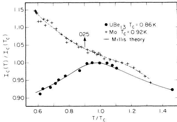
FIG. 2. Low-temperature I_c(T) for nonhysteretic junctions of Fig. 1. T is normalized to ingot T_c . Fall of I_c(T) in \text{UBe}_{13} contact indicates s -wave pair breaking by the bulk superconductivity. Dashed curve is a guide to the eye, while solid curve is obtained from Eq. (3), with \lambda = 2.8 , on the assumption I_c \propto \Delta_s \Delta_{\text{Ta}} .
