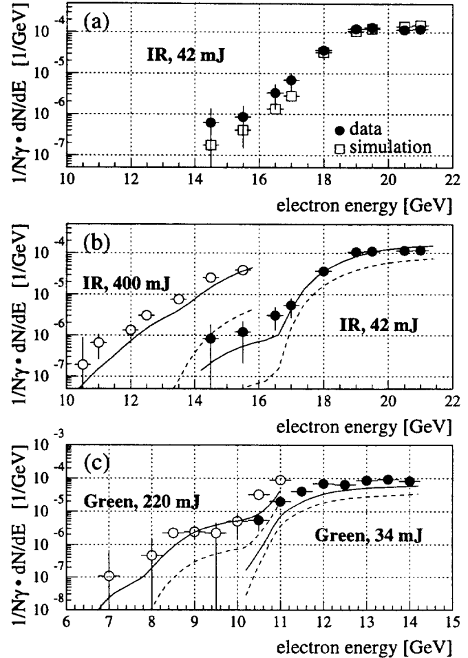
FIG. 4. Energy spectra of scattered electrons as observed in the ECAL calorimeter. (a): data and simulation for 42 mJ infrared laser pulses. (b),(c): Data (open and filled-in circles) and simulations (solid curves) for infrared (b) and green (c) laser pulses, scaled to standard values of the interaction geometry. The dashed lines show the simulation for multiple linear Compton scattering only.
