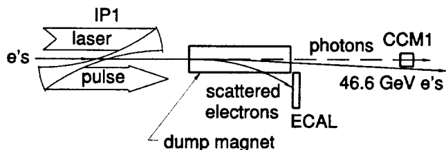
FIG. 2. Schematic drawing of the experiment.
