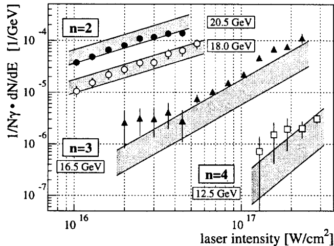
FIG. 5. The normalized yield of scattered electrons of energies corresponding to n = 2, 3 and 4 infrared laser photons per interaction point versus the intensity of the laser field at the interaction point. The bands represent a simulation of the experiment including 30% uncertainty in laser intensity and 10% uncertainty in N_\gamma .
