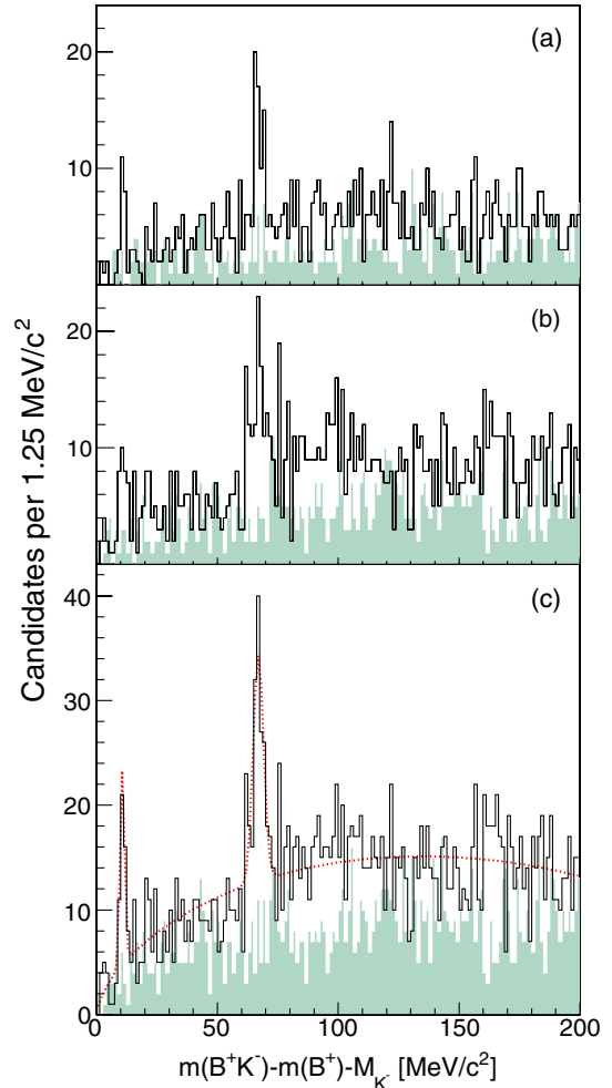
FIG. 1 (color online). Distribution of Q = m(B^+ K^-) - m(B^+) - M_K for the B_s^{**} candidates with (a) B^+ \rightarrow J/\psi K^+ , (b) B^+ \rightarrow \bar{D}^0 \pi^+ and (c) both B^+ channels combined. The dotted line shows the result of a fit with the sum of a background function and two Gaussians. The filled area shows the Q distribution for the wrong-sign combination B^+ K^+ .
