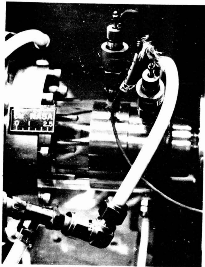
Figure 3. - Test bearing.
