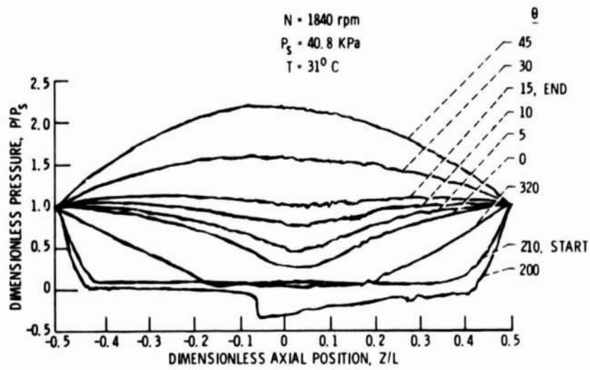
(c) N = 1840 \text{ rpm} ; P_s = 40.8 \text{ KPa} .
