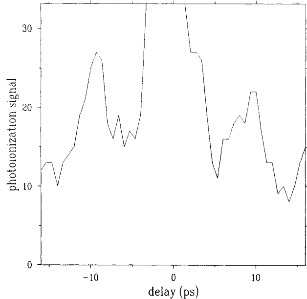
FIG. 2. The pump-probe photoionization signal as a function of the time difference between the two pulses. The numbers along the vertical axis are only for comparison with Fig. 3. For zero delay, the probe pulse directly ionizes the atoms excited by the pump pulse. At -9 and 9 ps the return of the wave packet is clearly observed.
