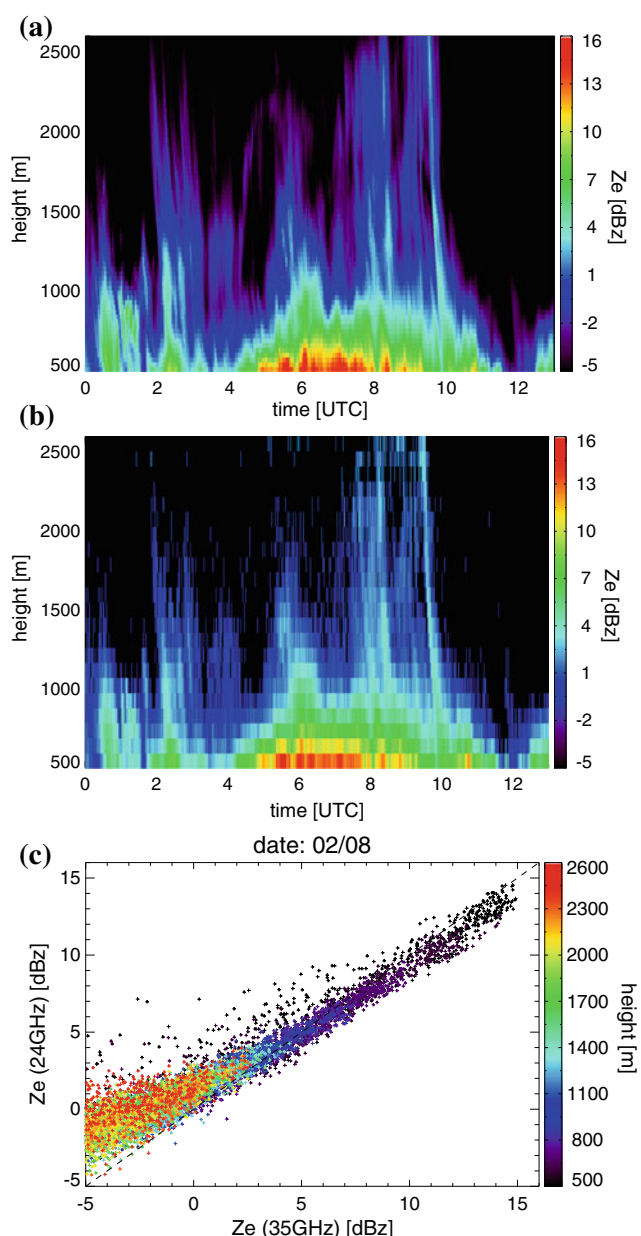
Fig. 7 Time–height cross sections of effective reflectivity factor Z_e (dBz) for a MIRA36 and b MRR on 08 February 2009. Z_e values from both radar systems and for all heights (color code) are plotted as scatter plot in c ; direct line is dashed. All MRR values have been converted into 35.5 GHz equivalent Z_e s according to Eq. 3. Note that the MIRA36 reflectivity values have been reduced to the MRR Z_e range
