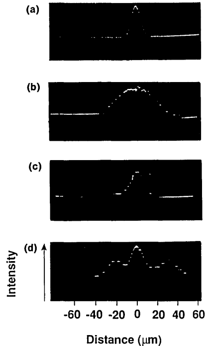
Fig. 2. Experimentally measured time-averaged beam profiles as a function of input power. (a) Input beam profile; (b) output beam profile, peak power 24 kW; (c) output beam profile, peak power 400 kW; (d) output beam profile, peak power 1.25 MW.
