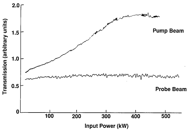
Fig. 4. Pump-probe measurements used to check on the mechanism of the nonlinearity. The top trace shows the transmission of the pump beam through an aperture, and the bottom trace shows the transmission of a delayed probe.
