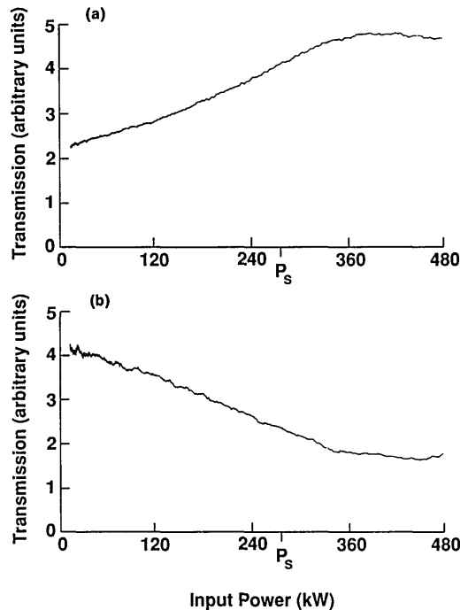
Fig. 3. Experimental measurements of the output power through an aperture of effective diameter 15 \mu\text{m} centered on (a) the output beam and (b) the wing of the output beam.
