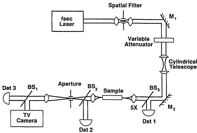
Fig. 1. Schematic of the apparatus used for the experiments. BS's, beam splitters; M's, mirrors.
