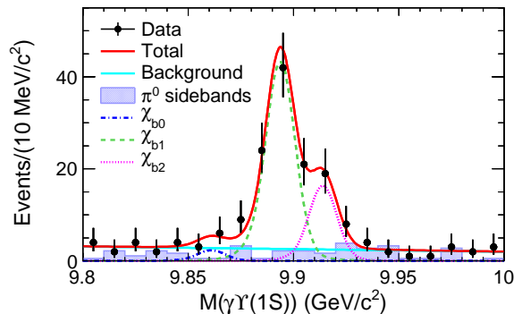
Figure 1. The \gamma\Upsilon(1S) invariant mass distribution for selected e^+e^- \rightarrow \pi^+\pi^-\pi^0\gamma\Upsilon(1S) candidate events. The shaded histogram is from normalized \pi^0 -sideband events. The fit to the \gamma\Upsilon(1S) invariant mass spectrum is described in the text. The solid curves are the best fit for the total fit and background shape; the dash-dotted, dashed and dotted curves represent the \chi_{b0} , \chi_{b1} and \chi_{b2} signals, respectively.
