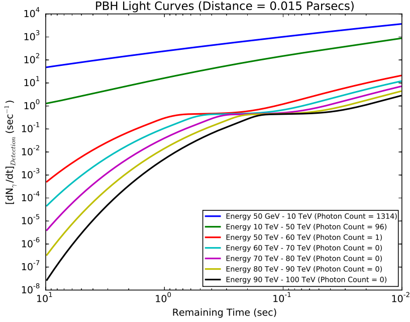
Figure 2: Simulated detection time profiles of a PBH burst at a distance of 0.05 light years observed by HAWC in multiple energy bands. Photon numbers detected in each energy band is shown in the legend.
