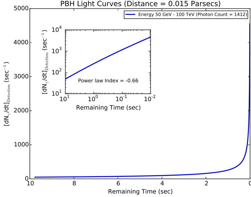
Figure 1: Simulated PBH Burst lightcurve observed by HAWC (at a distance of 0.05 light years) obtained by convolving with the HAWC effective area published in Ref [7]. This shape is also well described by a power law with a index of -0.66.
