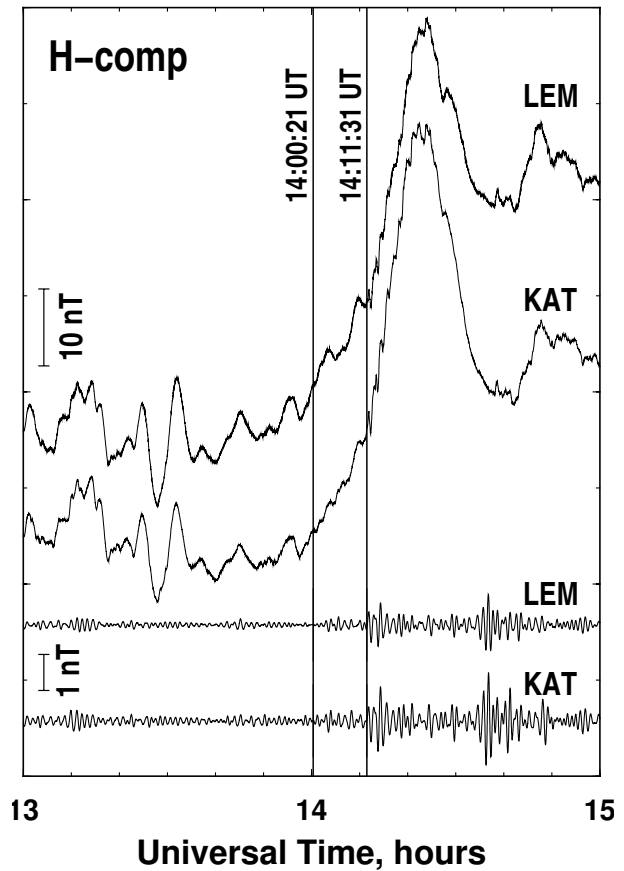
Fig. 8. One-second ground magnetometer data from the LEM and KAT stations in the 210MM array.
