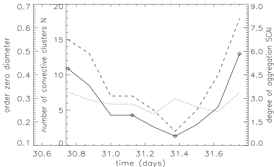
FIG. 5. (a) A sequence of CLAUS BT images over the African region 0°–20°N, 5°–30°E at (top left) 1800 UTC 30 Jul 2004, (top right) 0300 UTC 31 Jul 2004, (bottom left) 0900 UTC 31 Jul 2004, and (bottom right) 1800 UTC 31 Jul 2004. (b) Corresponding time series of N (dashed), \bar{D}_0 (dotted), and SCAI (plain). The diamonds on the SCAI curve correspond to the CLAUS images shown. Note that the magnitude of the SCAI range depends on the size of the domain under consideration (mainly owing to the dependence of N_{max} ).
