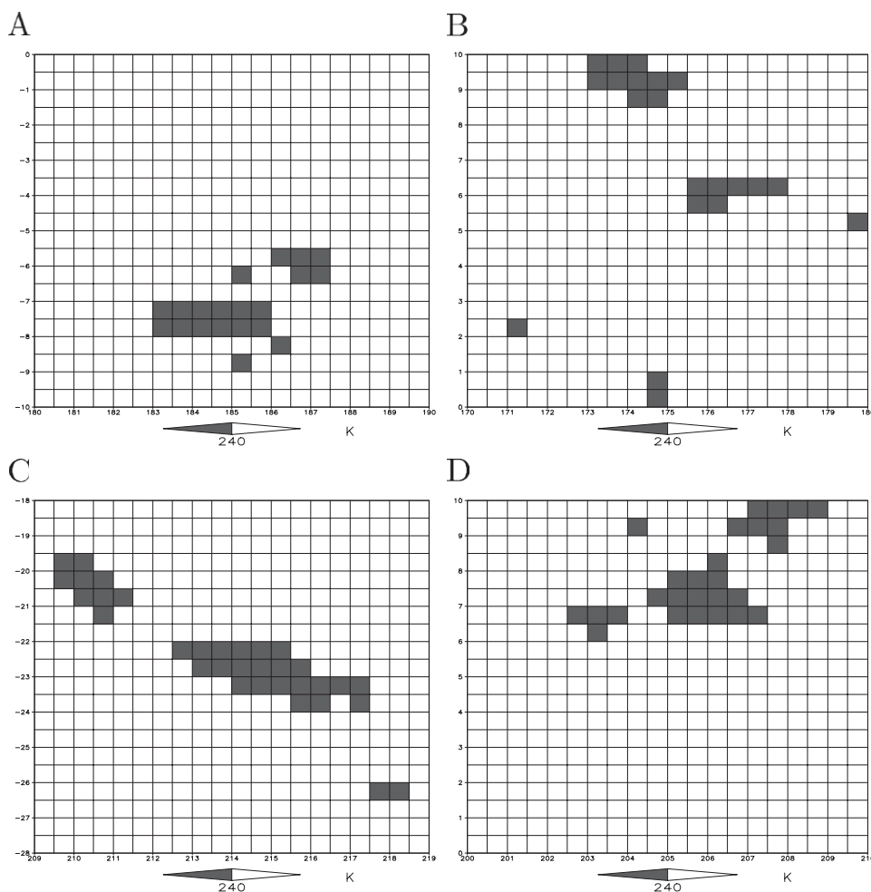
FIG. 2. Four examples of 10^\circ \times 10^\circ segmented domains: (a) 1200 UTC 11 Jul 1995, N = 5 , D_0 = 229 km, D_1 = 240 km, \text{SCAI} = 5.73 ; (b) 1200 UTC 21 Jan 2003, N = 5 , D_0 = 668 km, D_1 = 720 km, \text{SCAI} = 16.7 ; (c) 0600 UTC 21 Mar 1992, N = 3 , D_0 = 646 km, D_1 = 684 km, \text{SCAI} = 9.7 ; and (d) 0000 UTC 11 Jan 1988, N = 4 , D_0 = 334 km, D_1 = 344 km, and \text{SCAI} = 6.7 .
