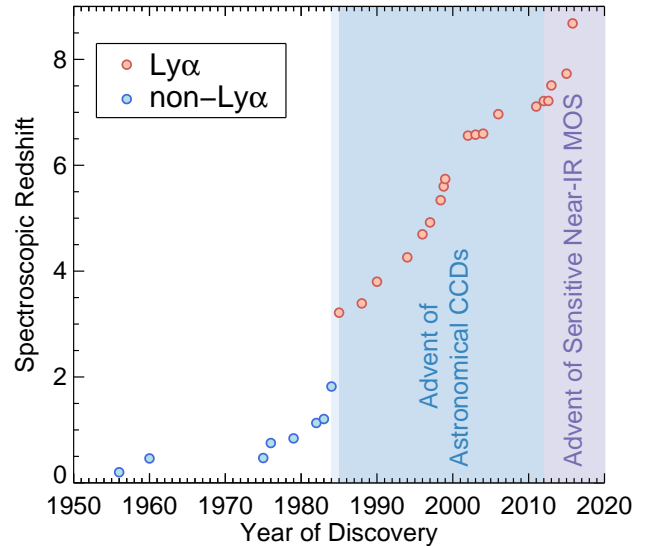
Figure 3. The highest redshift spectroscopically confirmed galaxy plotted versus the year of discovery. There are currently only three galaxies with robust spectroscopic redshifts at z > 7.5 : z = 7.51 from Finkelstein et al. (2013), z = 7.73 from Oesch et al. (2015b) and z = 8.68 from Zitrin et al. (2015). Data prior to 1999 were taken from the review of Stern & Spinrad (1999), with the references listed therein. Objects at later times come from Hu et al. (2002); Kodaira et al. (2003); Taniguchi et al. (2005); Iye et al. (2006); Vanzella et al. (2011); Ono et al. (2012); Shibuya et al. (2012); Finkelstein et al. (2013); Oesch et al. (2015b); Zitrin et al. (2015). The shaded regions denote roughly the time when CCDs became widely used, as well as when MOSFIRE (the first highly-sensitive near-infrared multi-object spectrograph) was commissioned on Keck. Major jumps in the most-distant redshift are seen to correspond with these technological advancements.
