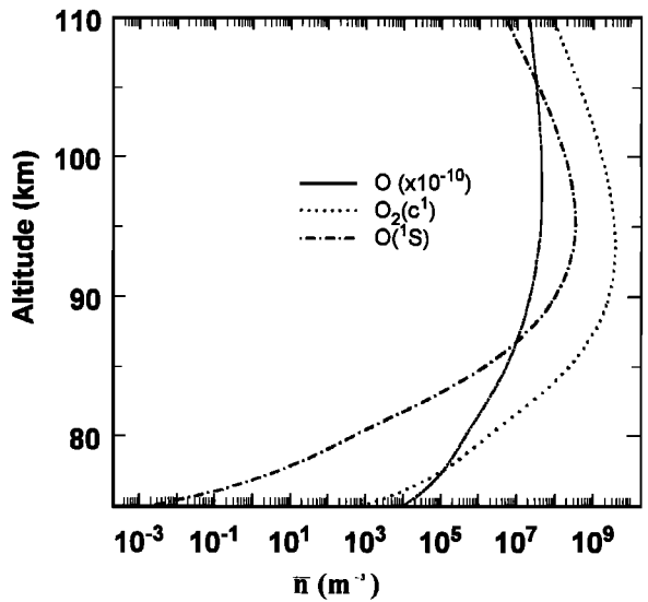
Figure 4. Height profiles of mean state minor species number densities \bar{n}(O) , \bar{n}(O_2[c^1\Sigma_u^-]) , and \bar{n}(O(^1S)) . \bar{n}(O) , is from the MSIS-90 model for April 10 at 18°N [Hedin, 1991]. The values of \bar{n}[O_2[c^1\Sigma_u^-]] and \bar{n}[O(^1S)] are from (7) and (8), respectively.
