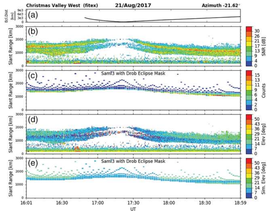
Figure 7. Comparison of simulated and measured data during the eclipse, where the Drob eclipse mask is used in the initialization of the SAMI3 model. (a) Eclipse geometry panel (distance [km]) of the eclipse center from radar [Ecl. Dist]; (b) measured signal-to-noise ratio (SNR) of signals received by the SuperDARN radar; (c) the number of simulated rays in each range gate; (d) measured angle of arrival (Elev) for returned scatter; and (e) simulated initial elevation angle (Sim. Elev) of ground scattered rays, assumed to be equivalent to angle of arrival of the reflected rays.
